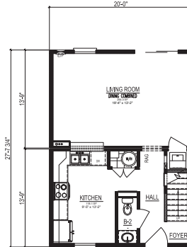
FIRST LEVEL FLOOR PLAN
